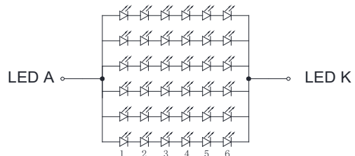
Backlight Circuit Diagram
