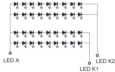
Backlight Circuit Diagram
