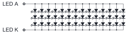
Backlight Circuit Diagram
