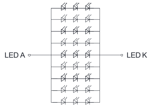
Backlight Circuit Diagram
